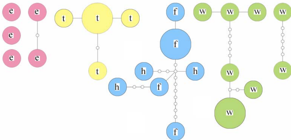
FIG. 3. Haplotype networks of Allactaga spp. (27 individuals), based on 616 bp of the cytochrome oxidase subunit I gene ( Cox1 ). Networks were not joined if haplotypes were separated by more than 9 mutations. Each circle represents one haplotype. (pink circles (e): A. elater , yellow circles (t): A. toussi , blue circles (h, f): A. hotsoni and A. firouzi , green circles (w): A. williamsi ).
